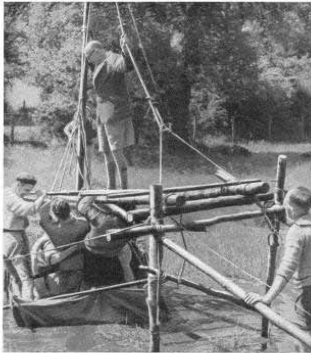
A RAFT NEGOTIATES A DERRICK BRIDGE
