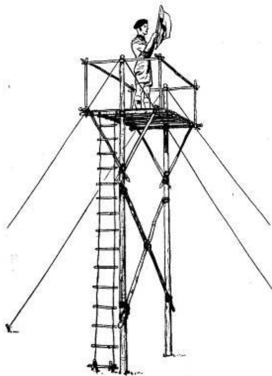
Stilt Tower.
