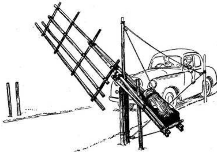
Counterpoise Gate.
